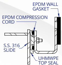
TOP SEAL
