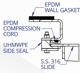
SIDE SEAL
