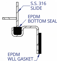
BOTTOM SEAL
