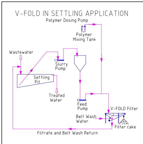
Settled winery sludge pumped to a “Day Tank” then to a V-FOLD filter
