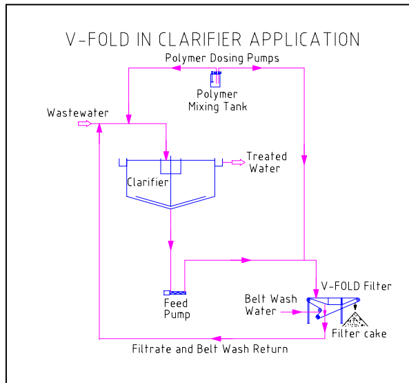
Clarifier underflow pumped directly to a V-FOLD filter
